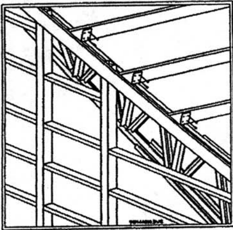
7 ENDPOST
